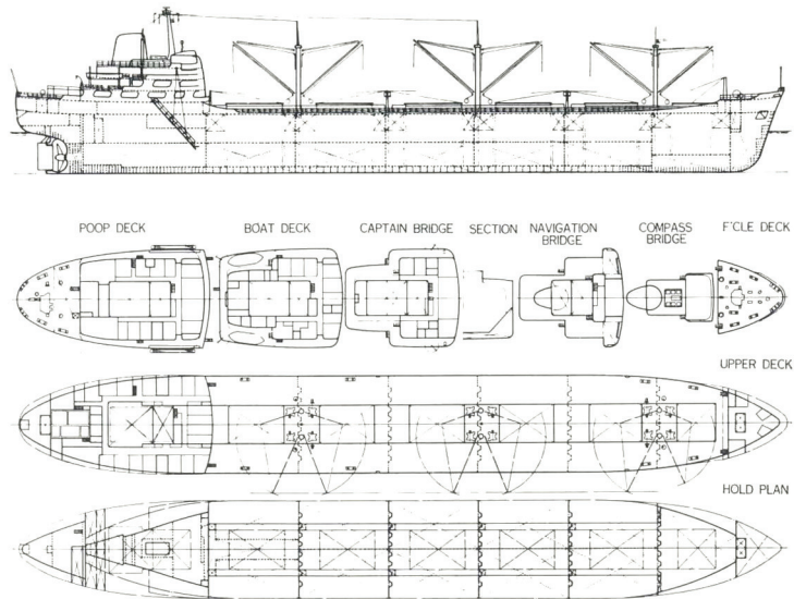
21,000 L.T. D. W. TURBINE BULK CARRIER "LINDA" GENERAL ARRANGEMENT
